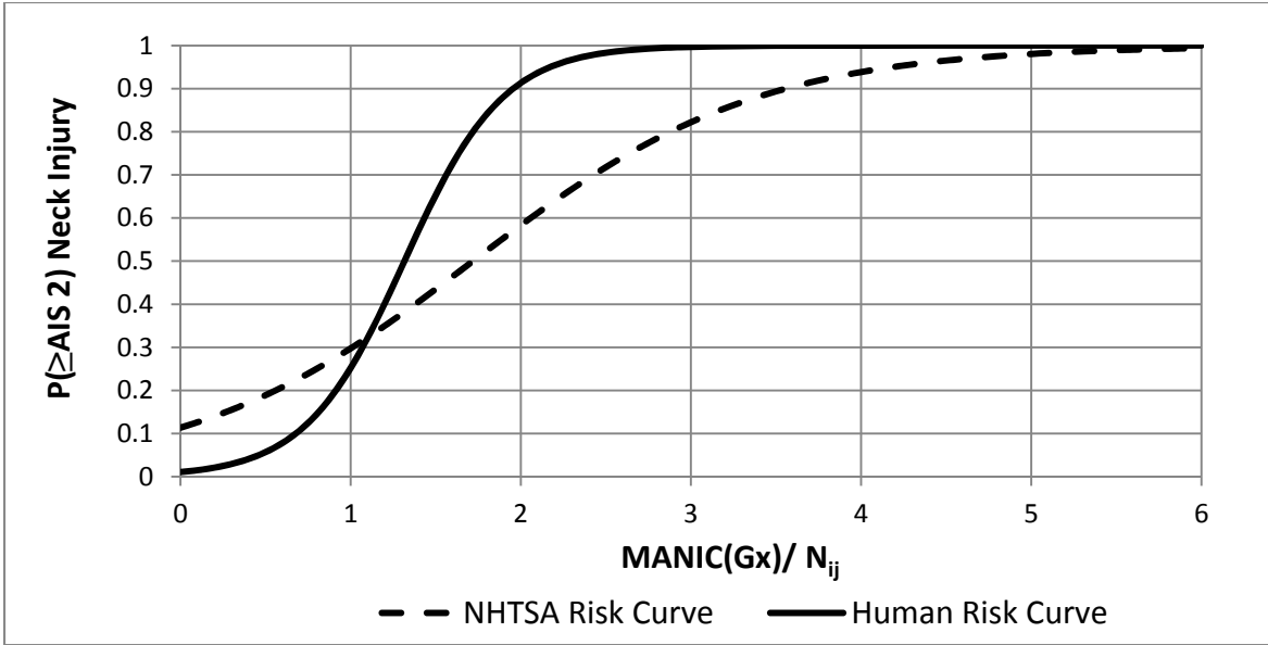
Figure 4. Probability of AIS 2 or Greater NHTSA and Human Neck Injury Risk Curves (Parr et al., 2013)
